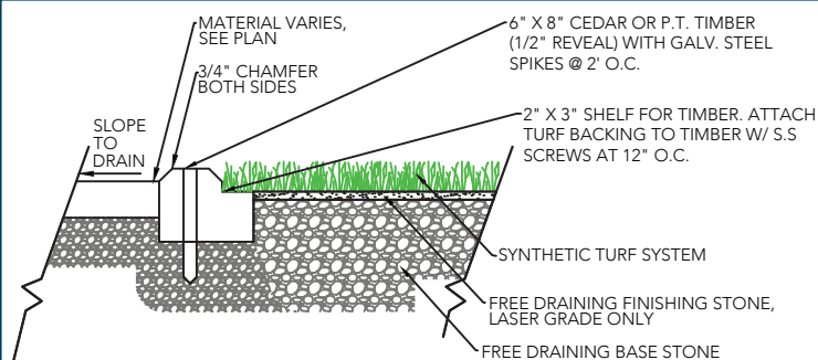
NAILER BOARD
